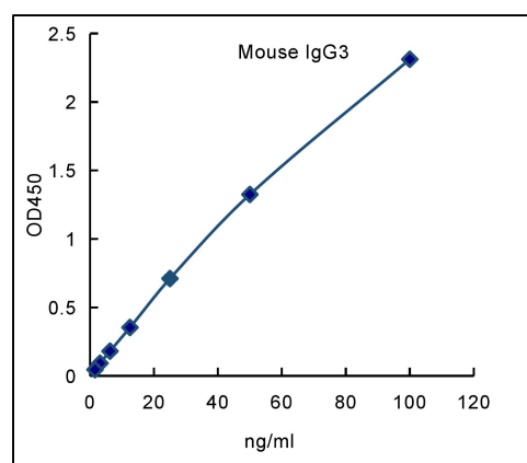
Plot mouse IgG3 standard curve
