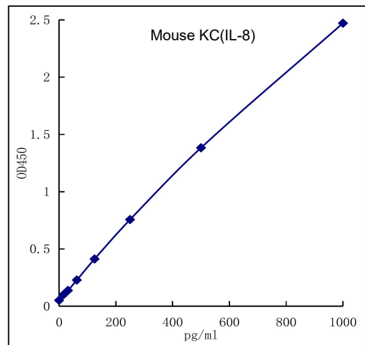
Plot Mouse KC(IL-8) standard curve
