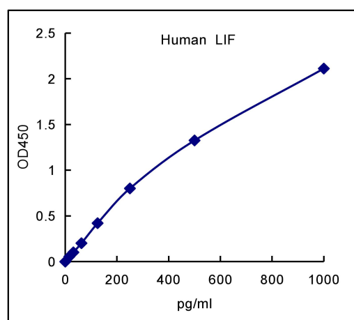
Plot human LIF standard curve
